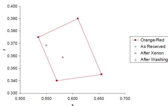
Chromaticity - ISO 20471:2013
